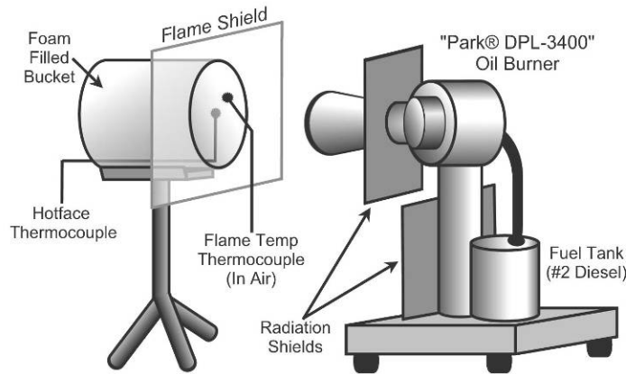
Figure -3 "Oil Burner" and test pail set-up
