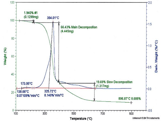
Figure-2 TGA of FR-3706 in Nitrogen
