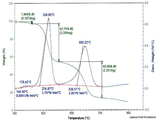
Figure-1 TGA FR-3706 in Air
